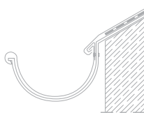
Suspended gutter
