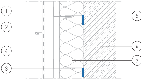
Horizontal section through elZinc® titanium zinc facade with metal substructure
